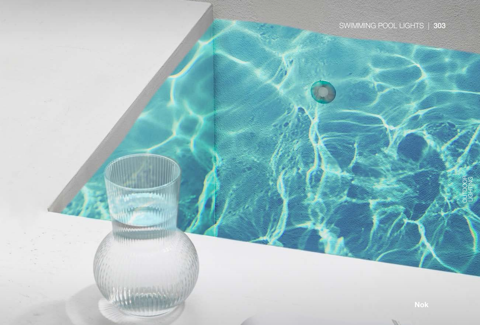
Nok Swimming Pool Light Stainless Steel/Glass SMD LED 196lm; 4000K; 3W IP68; CRI >80 Dia. 44 x H170 mm
